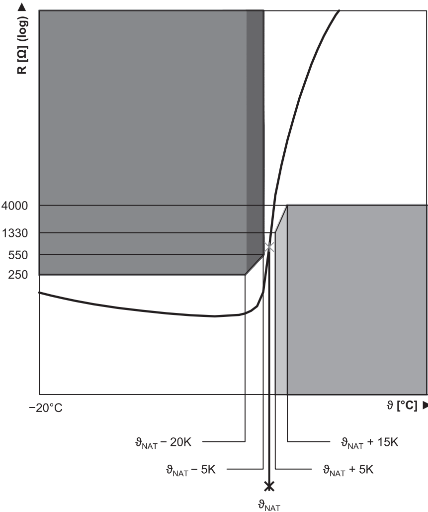
Fig. 2: PTC thermistor curve (single thermistor)
