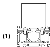
(1) internal profile with cover bands
