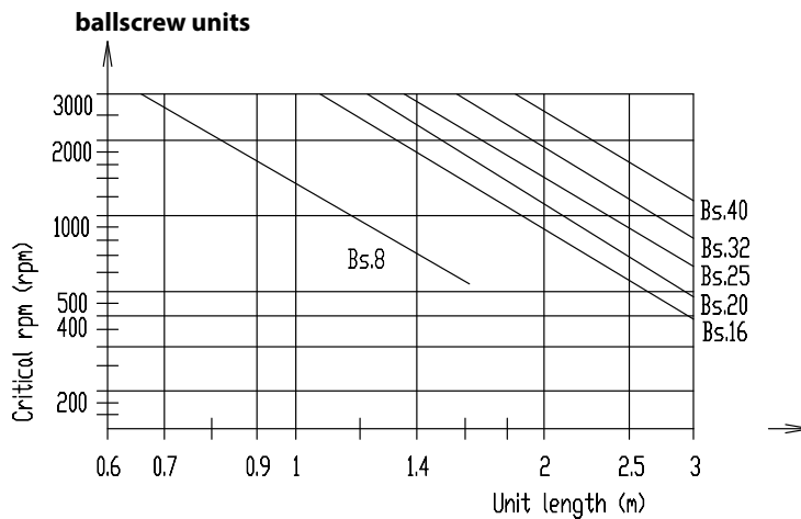
Diagram for maximum rpm of spindle units
